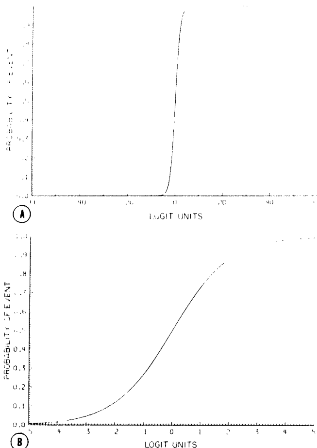
Fig. 2. Nomograms of the logistic equation. A. The nomogram is presented with \pm 60 logit units along the horizontal axis. The equation and the nomogram indicate a specific probability for each specific total logit unit. B. Nomogram of the same equation, portrayed with \pm 5 logit units along the horizontal axis. The same specific probability is denoted by each specific total logit unit, and the relation between the two as portrayed in the nomogram only seems to be different.
